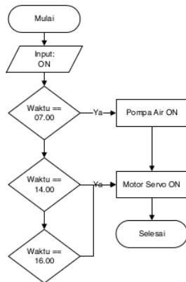
Gambar 5. Flowchart Prototype Alat Otomatis
