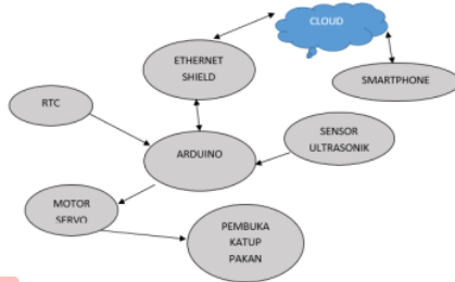
1 Gambar 7. Topologi Cloud Alat otomatis
