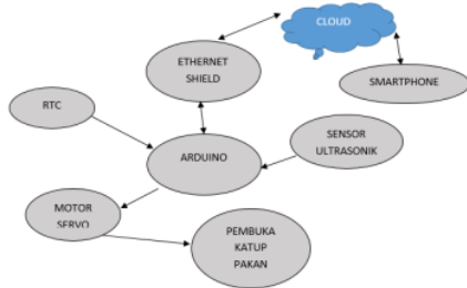
Gambar 7. Topologi Cloud Alat otomatis
