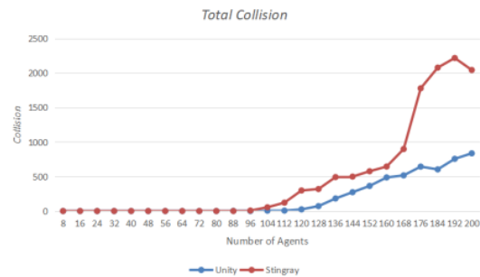
Fig 12. Collision Occured in Narrowpassage Scenario
