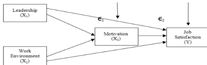
Figure 1. Research Model
