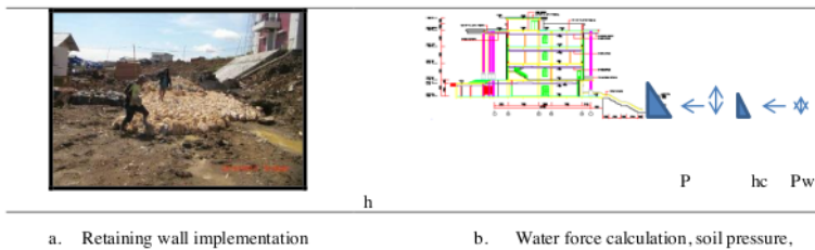
Figure 5. counterfort, retaining wall by utilizing stairs and floor plate unity with tie beam and pile cap
