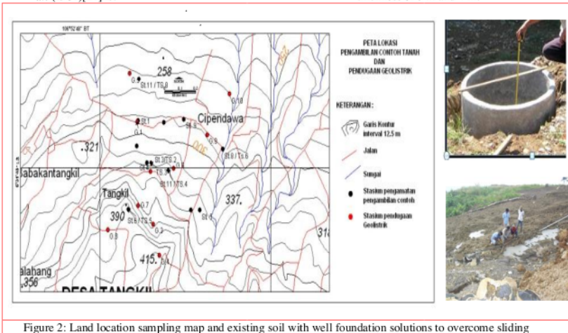
Figure 2: Land location sampling map and existing soil with well foundation solutions to overcome sliding
