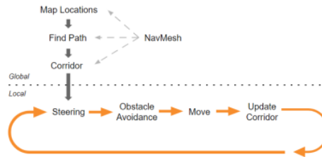
Fig 3. Navigation system of agents movement on Unity3D[10]
