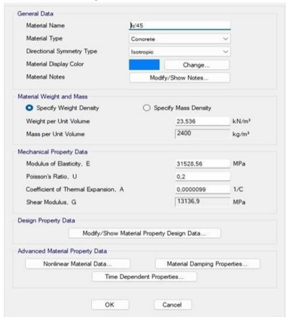
Gambar 6.15 Define Material Beton
