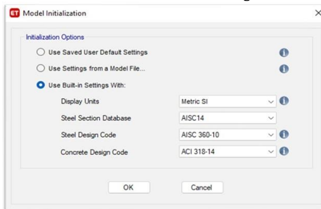
Gambar 6.9 Model Initialization
