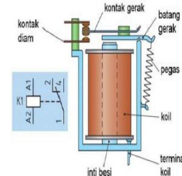
Gambar 5 Relay [5]
